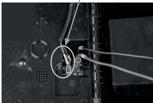
Fig. 4b Connection solar panel - for solar panel 5W or 10W - cable entry on the back of the device of the housing and connect in the housing lid.
