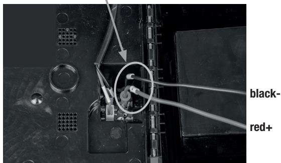
Fig. 4c Connection battery -for 9 VOLT DRY BATTERY or recharging 12V battery Make sure that the polarity is correct!
